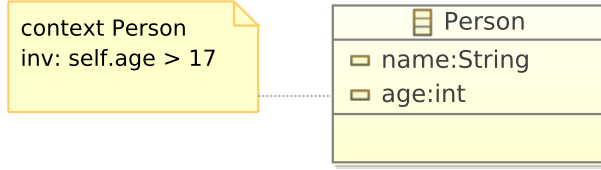
Figure 3: A simple OCL example
