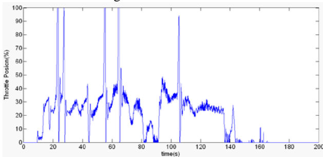
Fig.23 Throttle position
